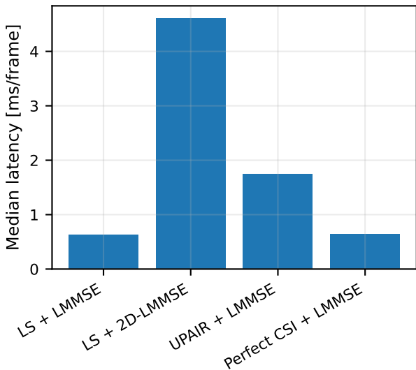
U2: receiver latency Wide-deep d128-b6-r2
